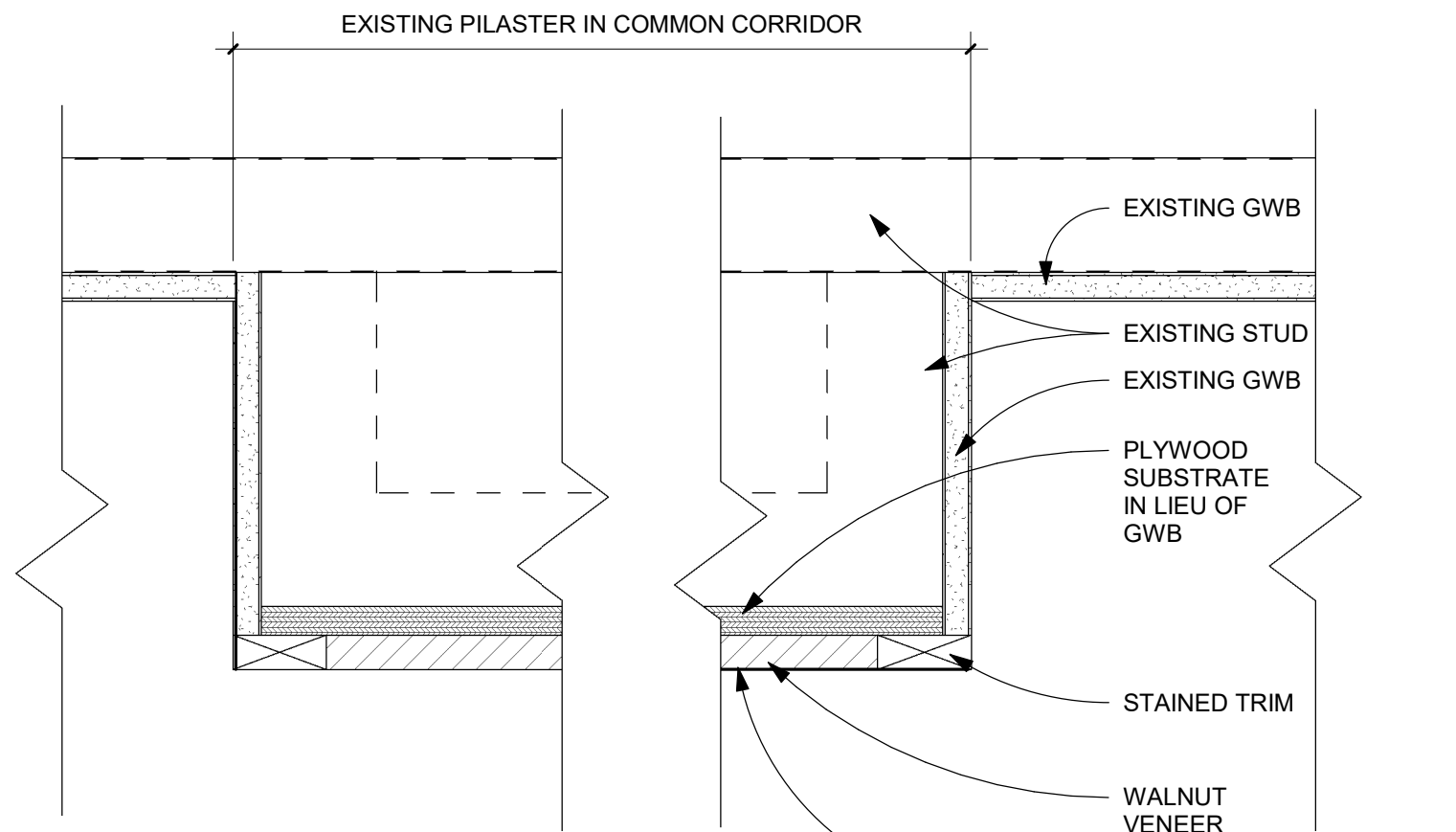
1 i-6.01 ADD ALTERNATE - CORRIDOR WOOD VENEER TRIM HEAD/JAMB DETAIL 3" = 1'-0"
