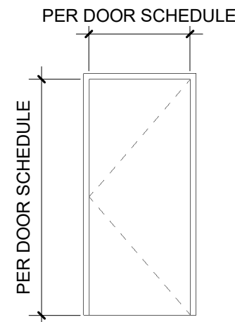
A SOLID CORE WD DOOR WITH HM FRAME
